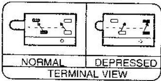
BRAKE SWITCH 4-TERMINAL
