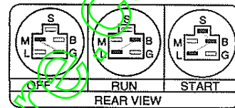
IGNITION SWITCH
