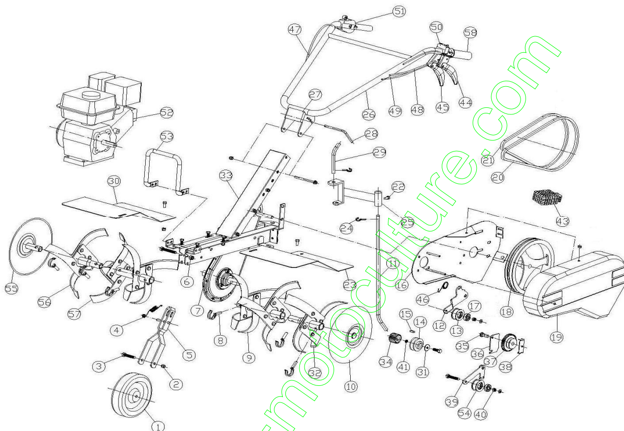
FY-ST75A Tiller part list
