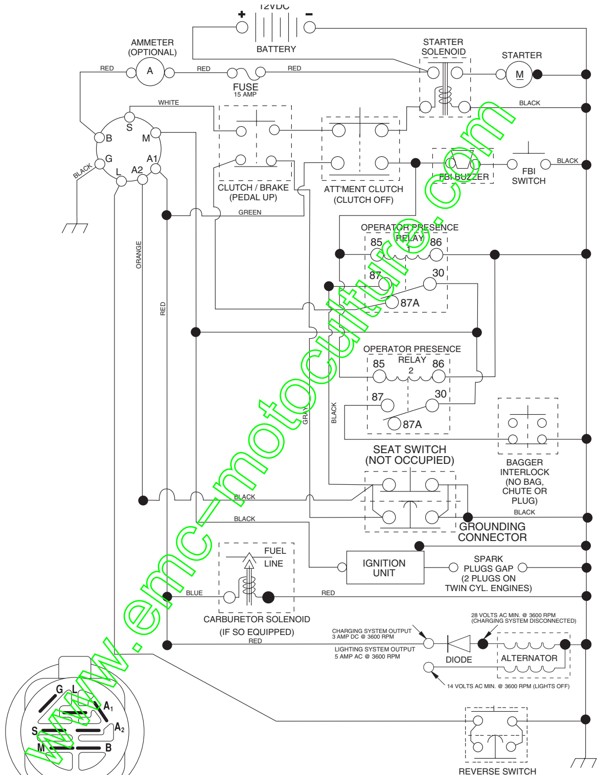
IGNITION SWITCH
