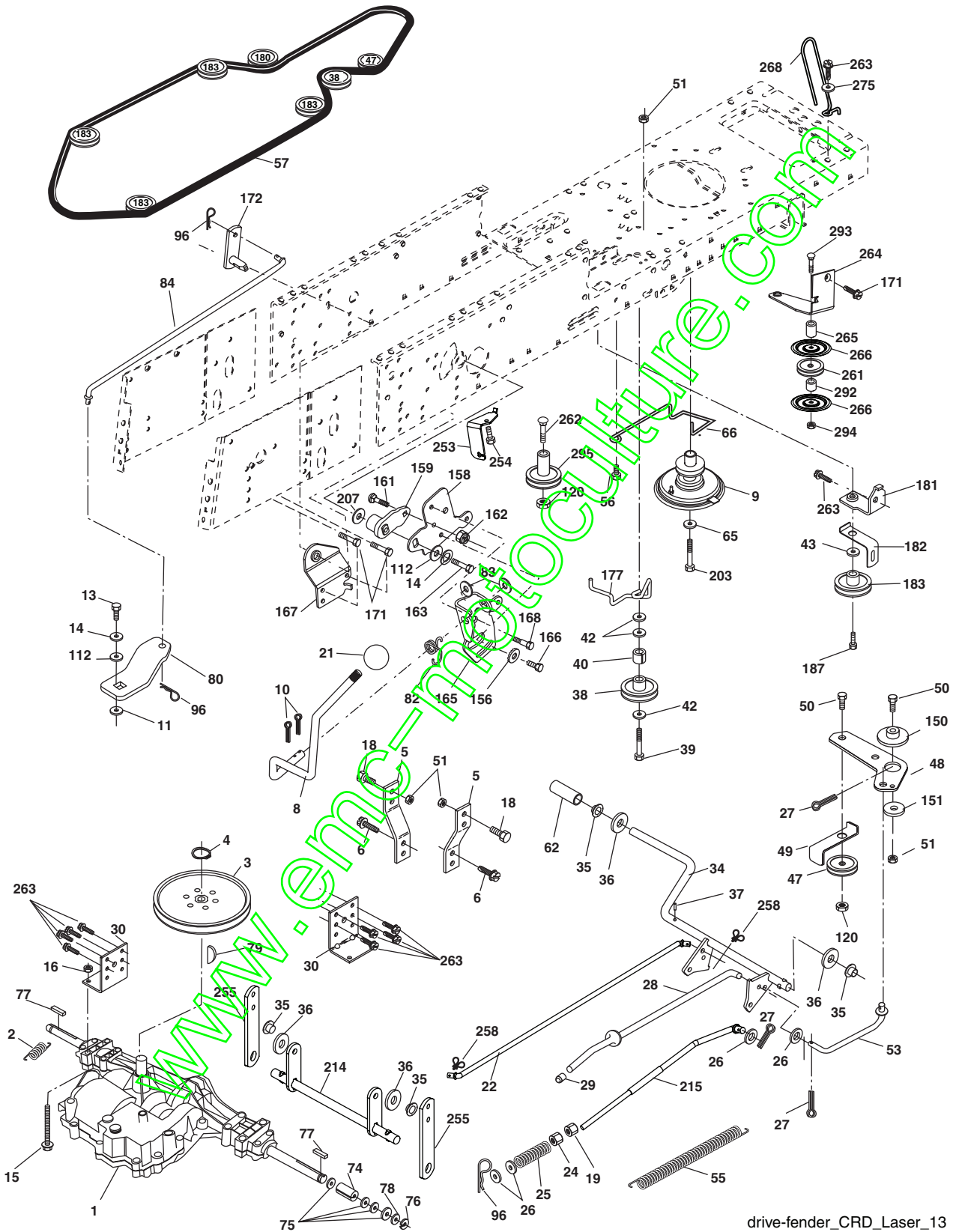
drive-fender_CRD_Laser_13
