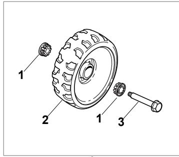
BUSHING Version - Ø 165
