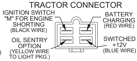
TRACTOR CONNECTOR
