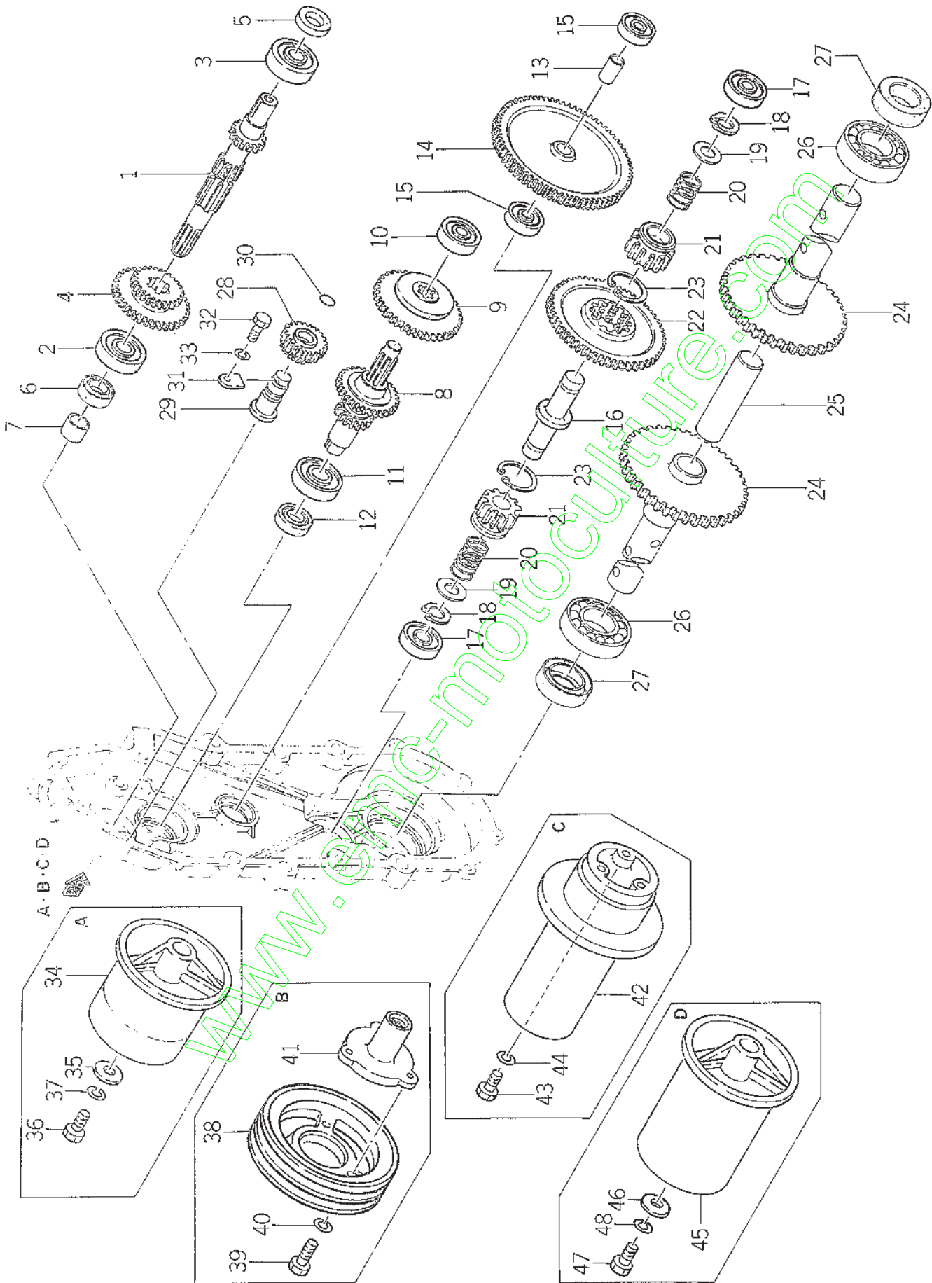
Fig.3 TRANSMISSION GEAR
