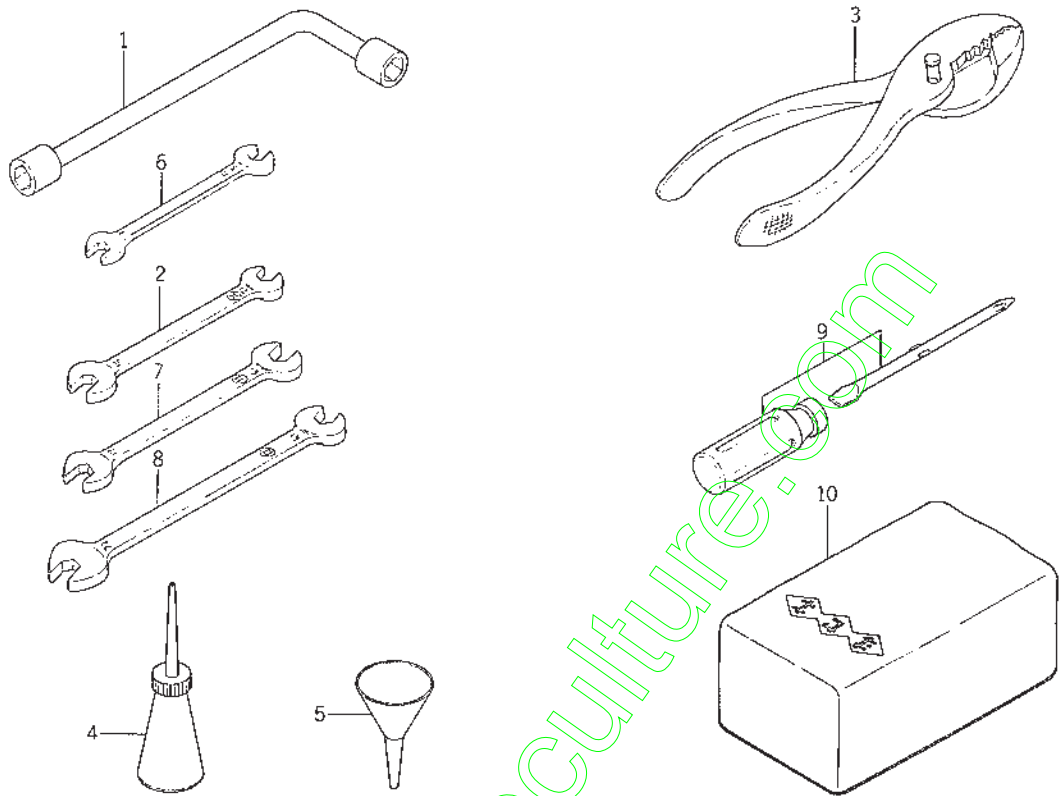
Fig.12 TOOLS
