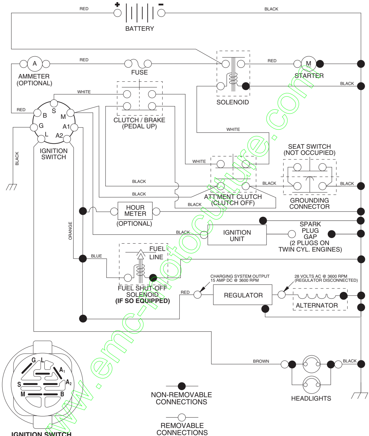
IGNITION SWITCH
