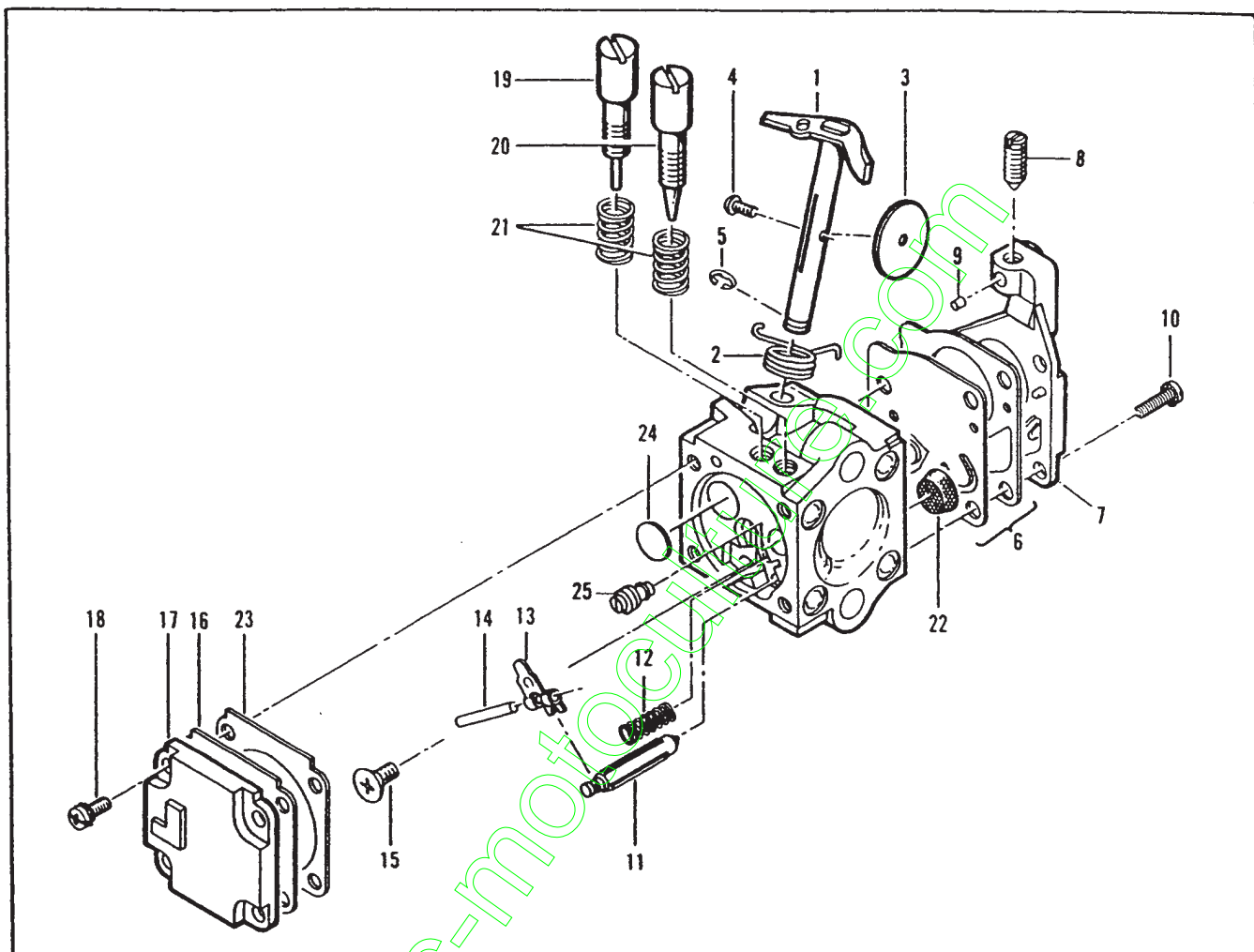
Figure 3. Carburetor Assembly.
