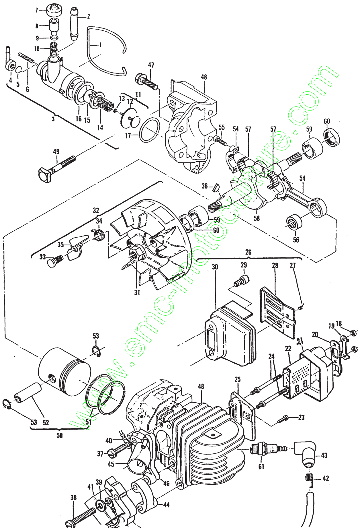
Figure 4. Powerhead Assembly.
