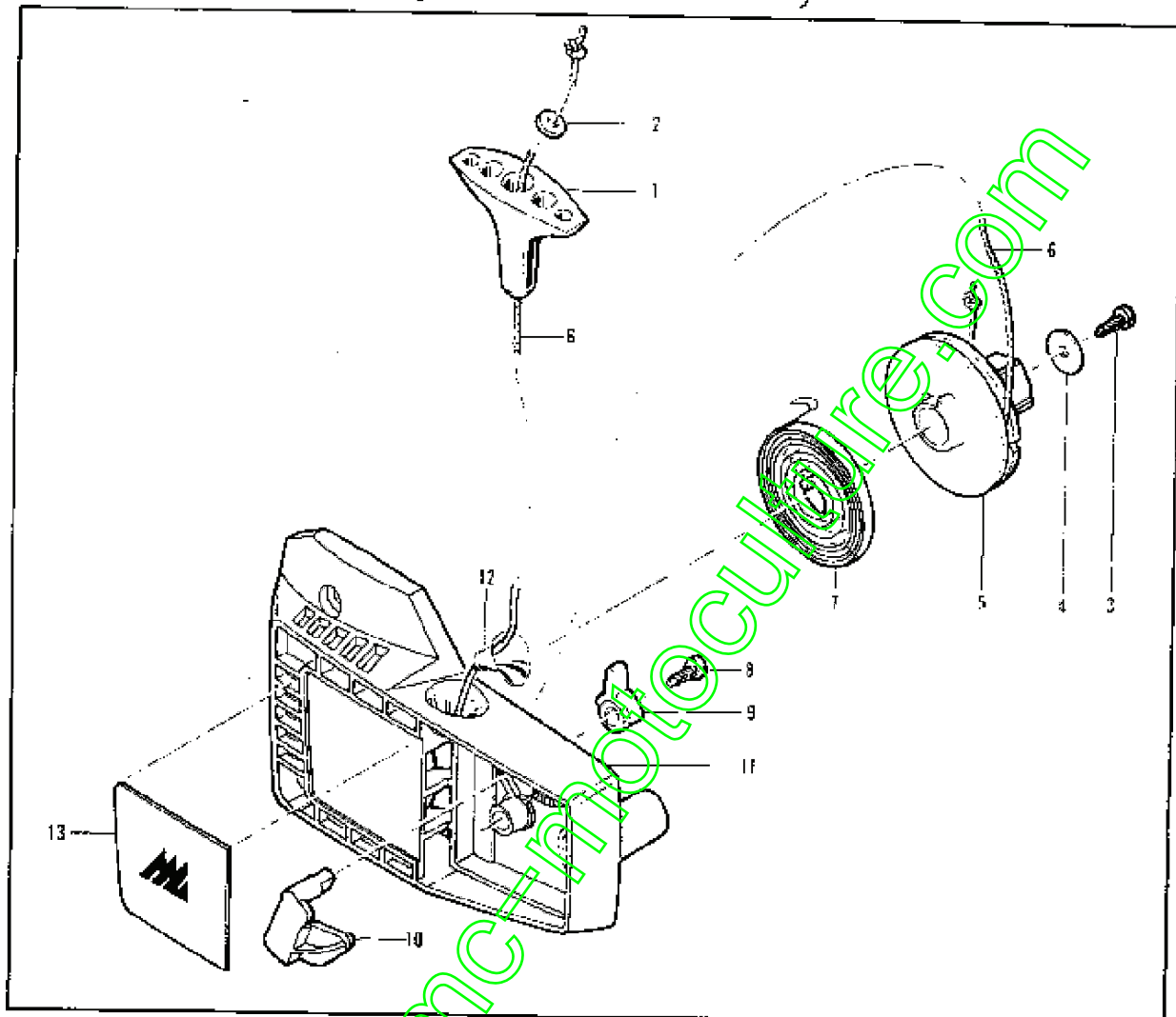
Figure 4. Starter Assembly
