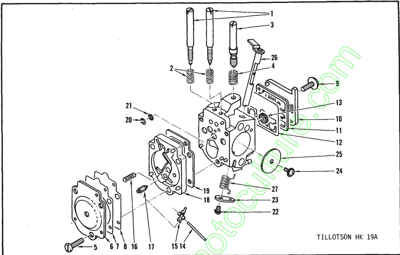
Figure 2. Carburetor Assembly
