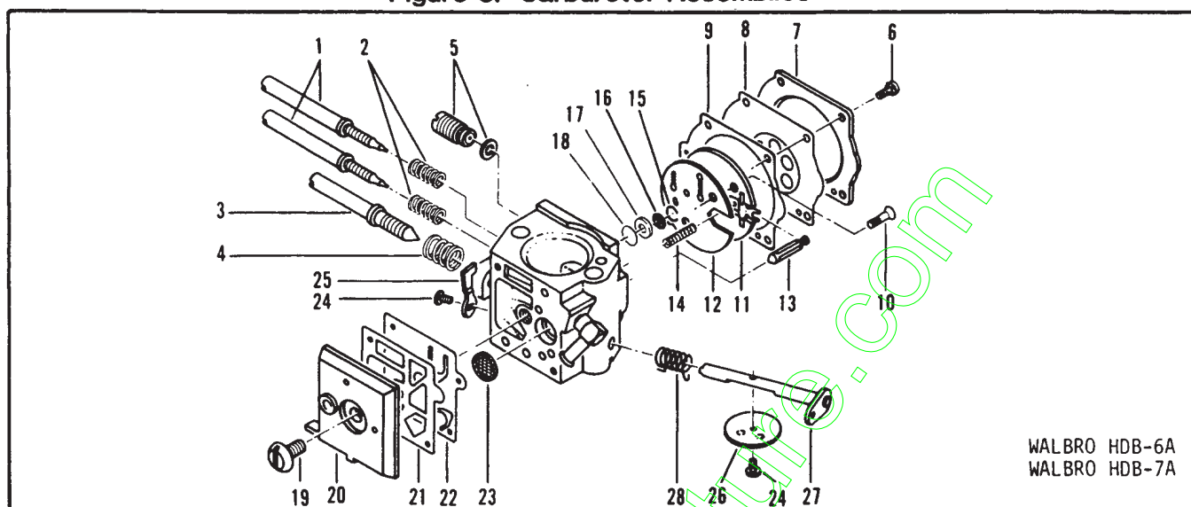
Figure 3. Carburetor Assemblies
