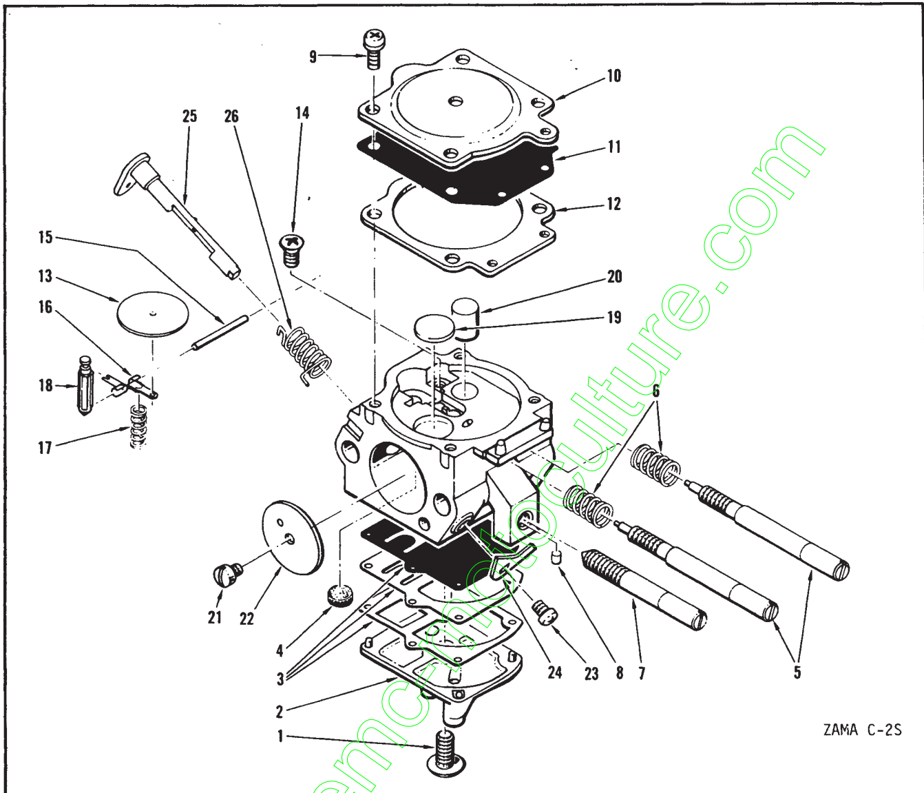
Figure 4. Carburetor Assembly.
