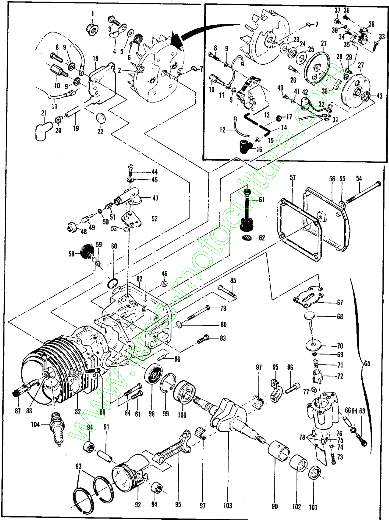
Figure 6. Powerhead Assembly
