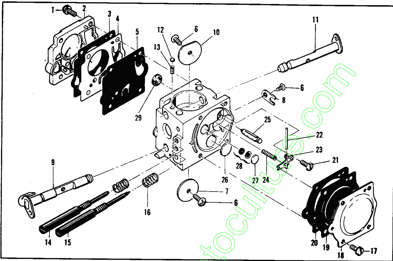
Figure 4. Carburetor Assembly
