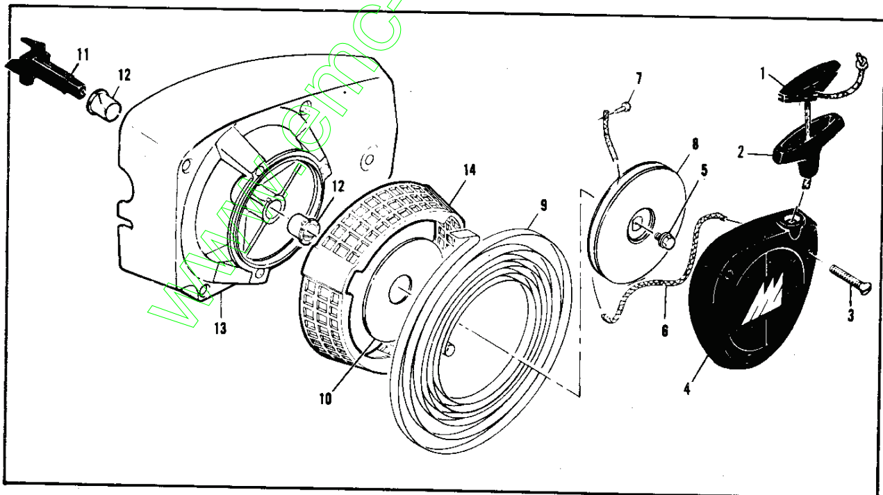
Figure 3. Fan Housing & Starter Assemblies
