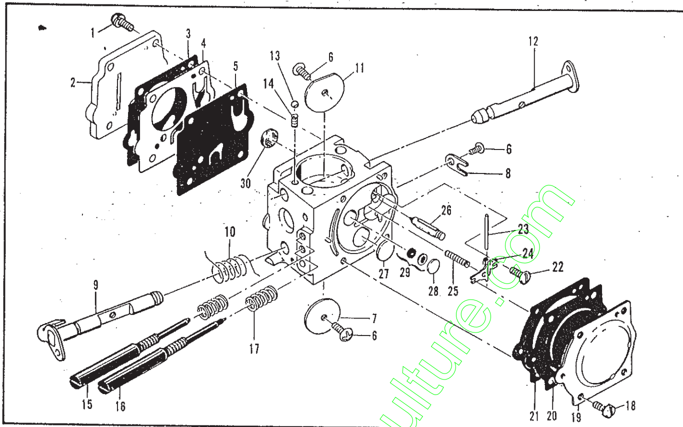
Figure 6. Carburetor Assembly
