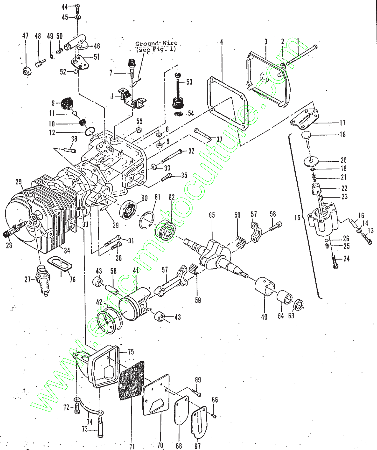
Figure 9. Powerhead & Oiler Assemblies.
