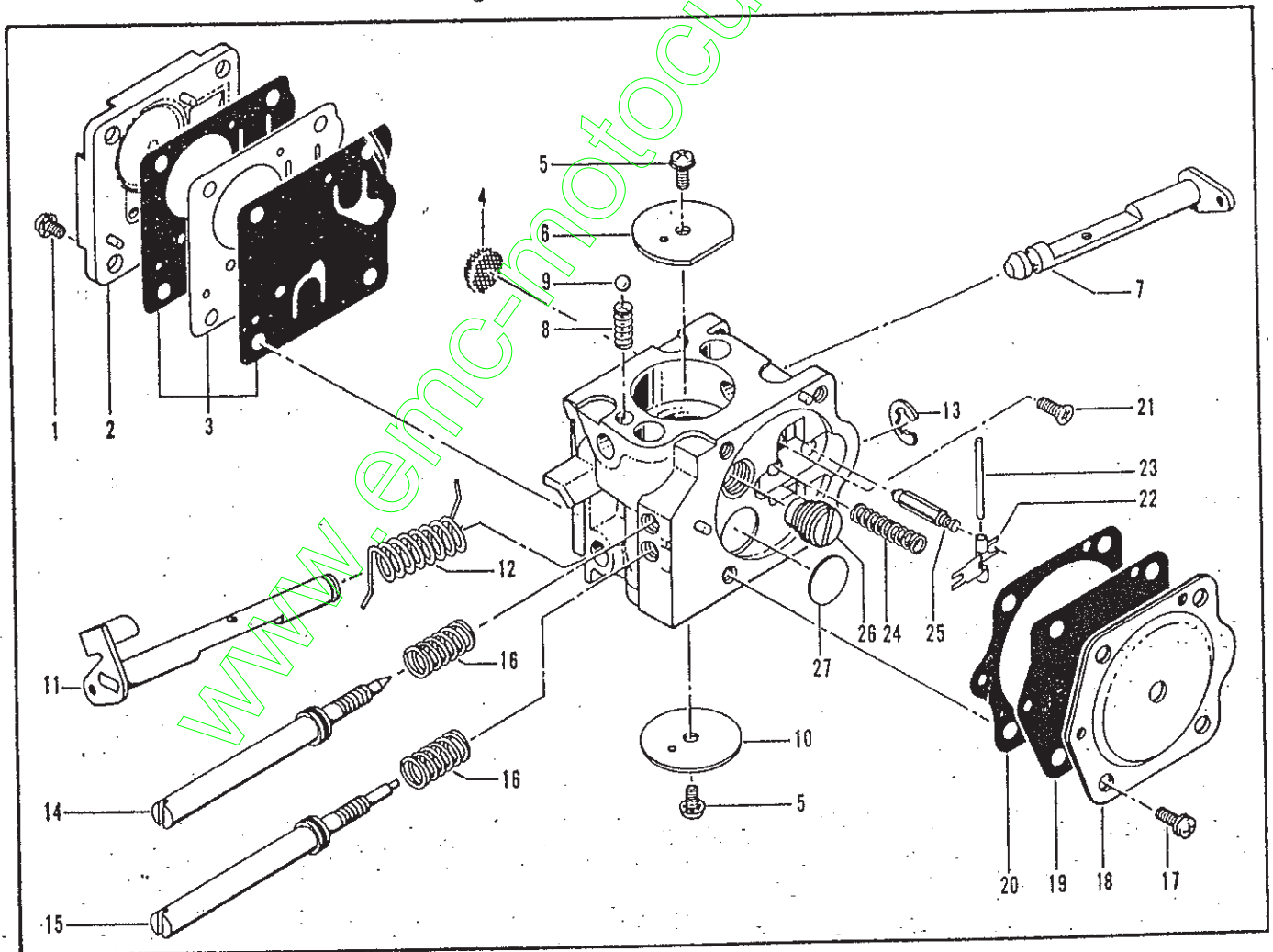
Figure 5. Carburetor Assembly
