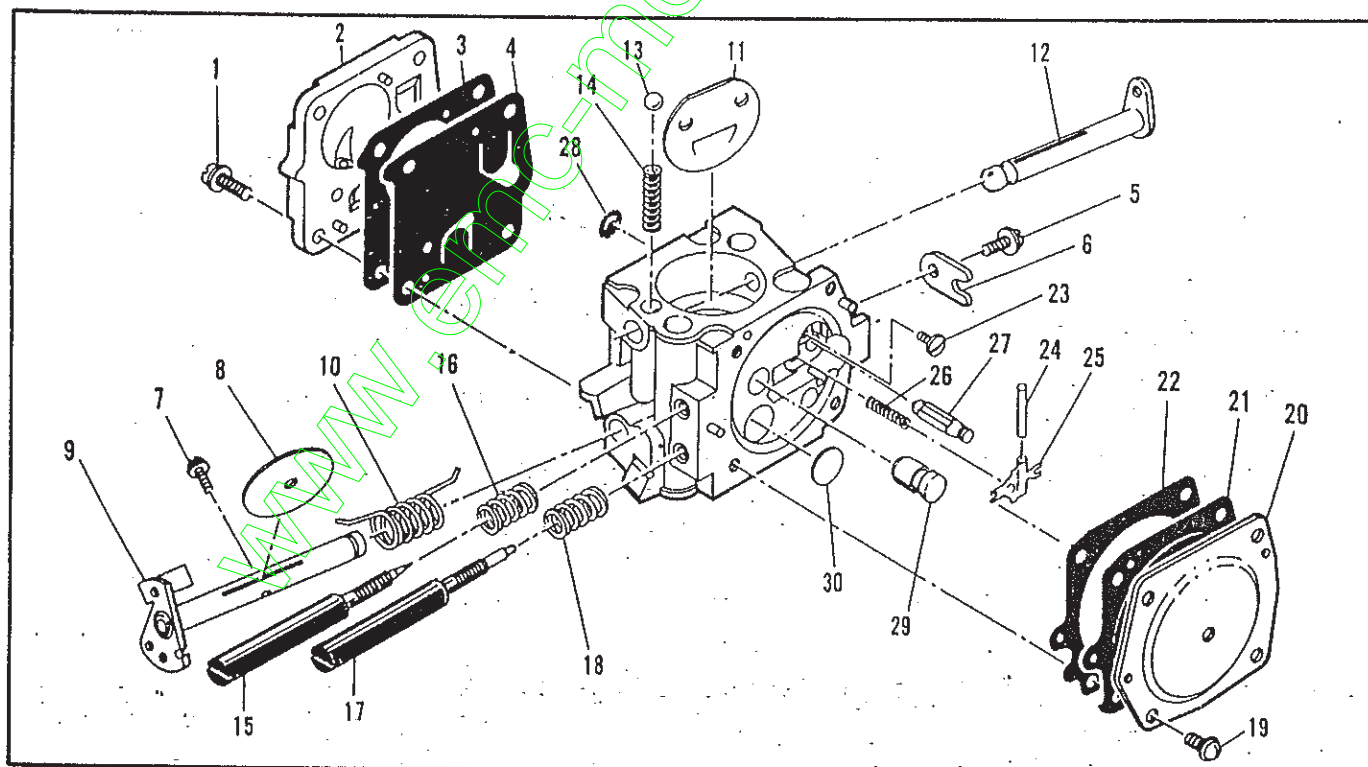
Figure 7. Carburetor Assembly
