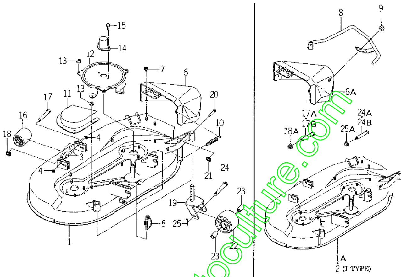
FIG. 21 DECK AND COVER SYSTEM
