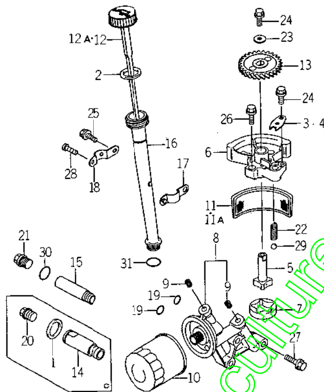
FIG. 4 LUBRICATION EQUIPMENT
