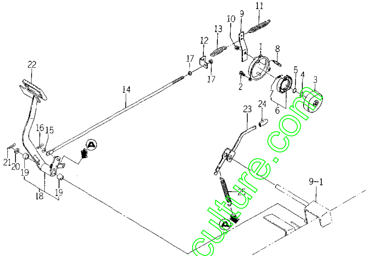
FIG. 7 BRAKE SYSTEM
