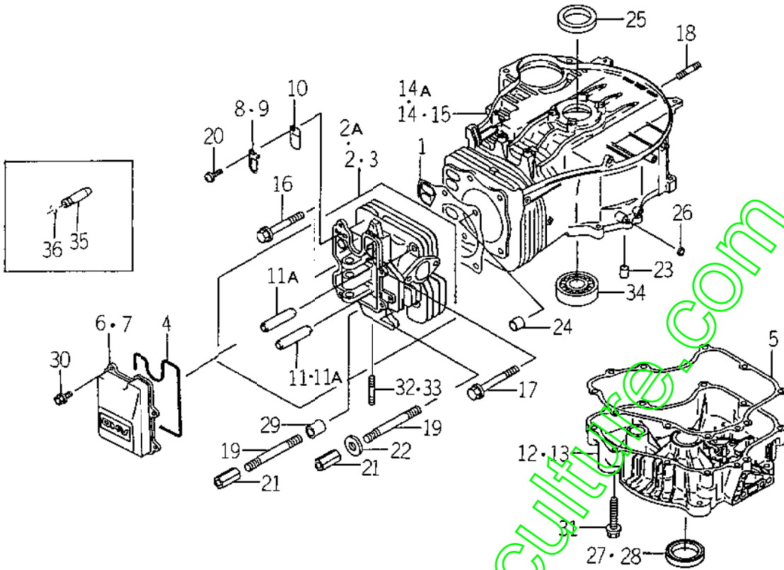
FIG. 1 CYLINDER CRANKCASE
