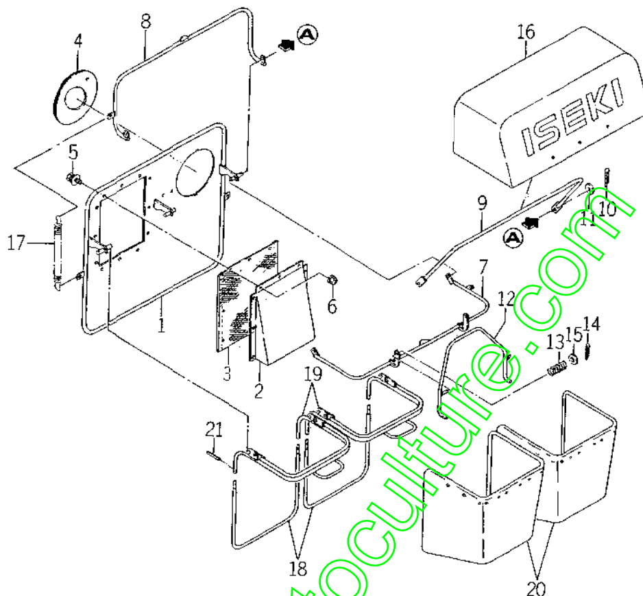
FIG. 24 PANEL AND FRAME SYSTEM
