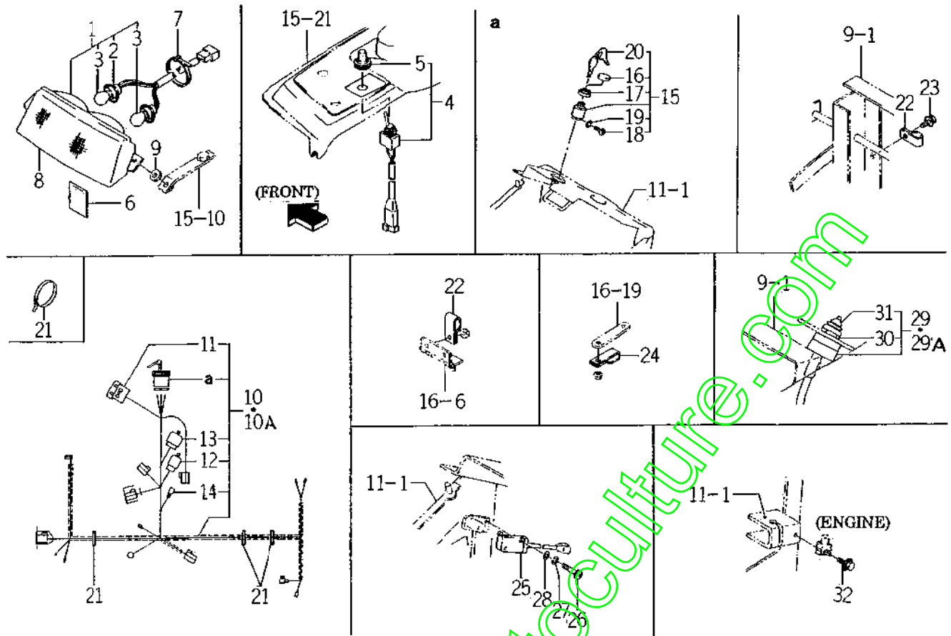
FIG. 17 ELECTRICAL SYSTEM
