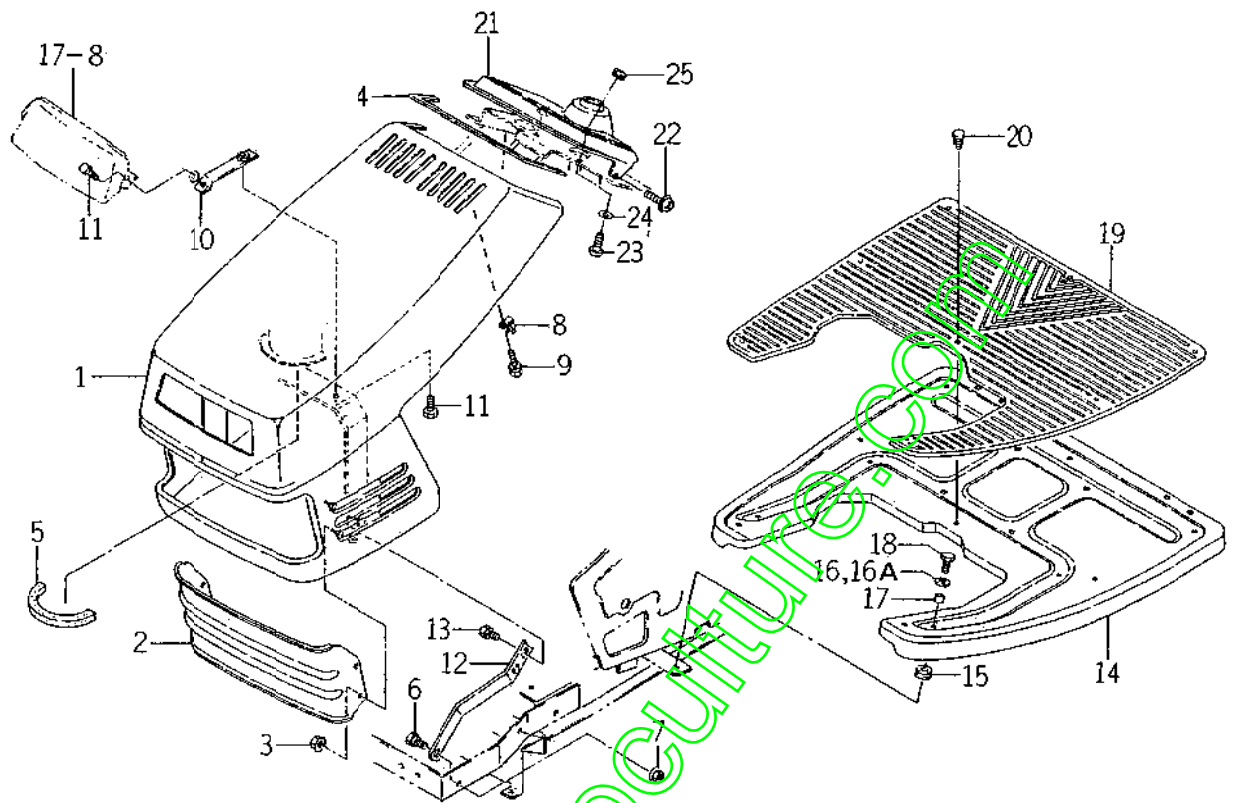
FIG. 15 HOOD AND PANEL SYSTEM
