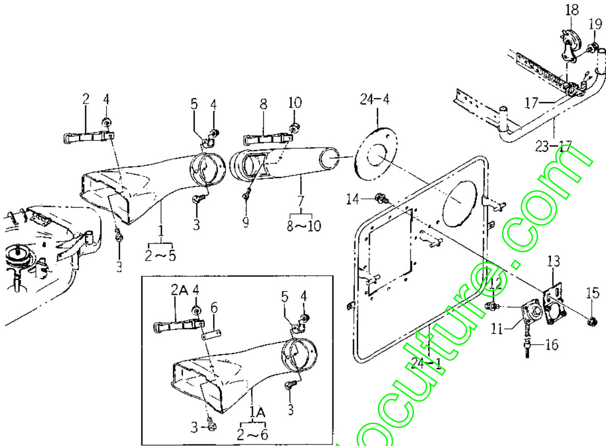
FIG. 25 COVER AND PIPE SYSTEM
