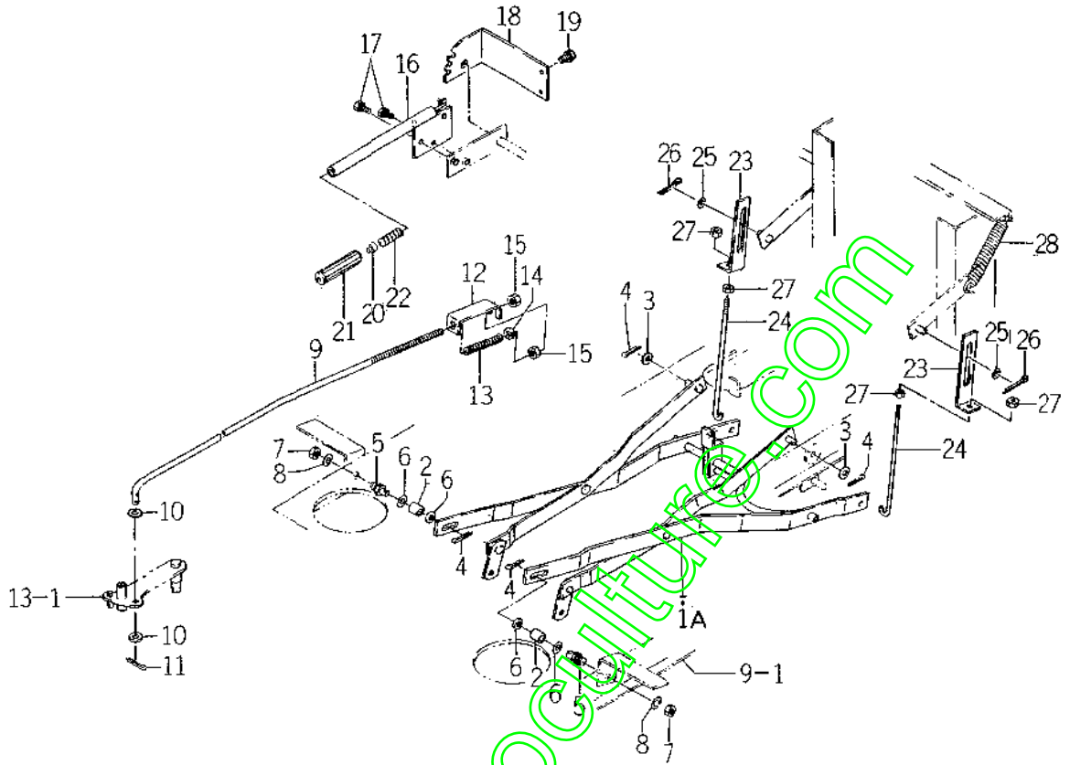
FIG. 14 LINK SYSTEM
