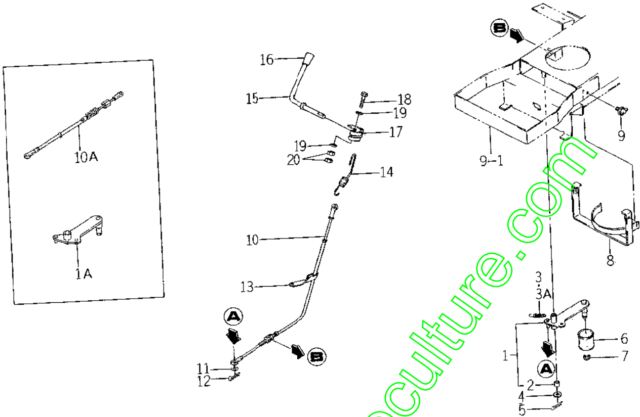
FIG. 13 P.T.O. SYSTEM
