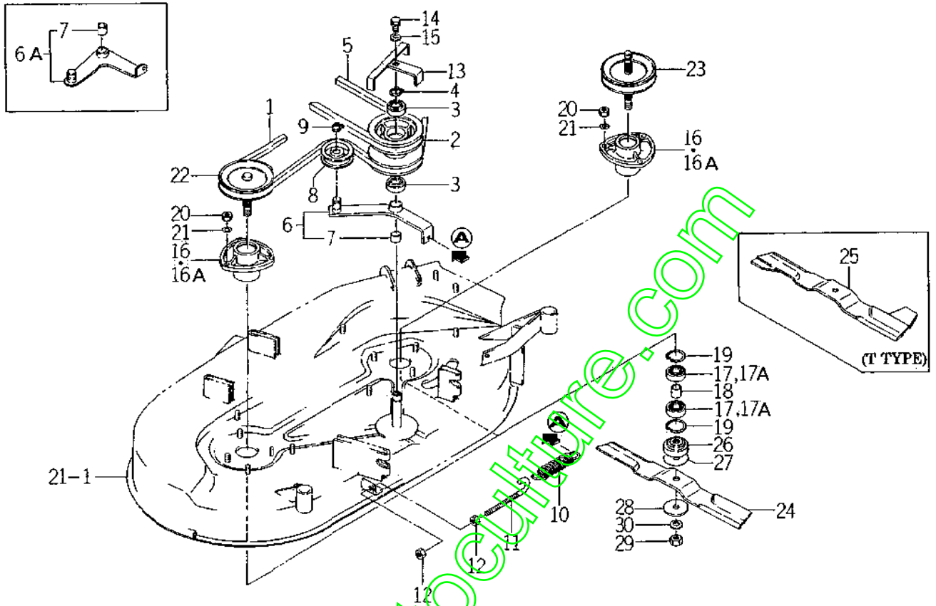
FIG. 20 DRIVING SYSTEM
