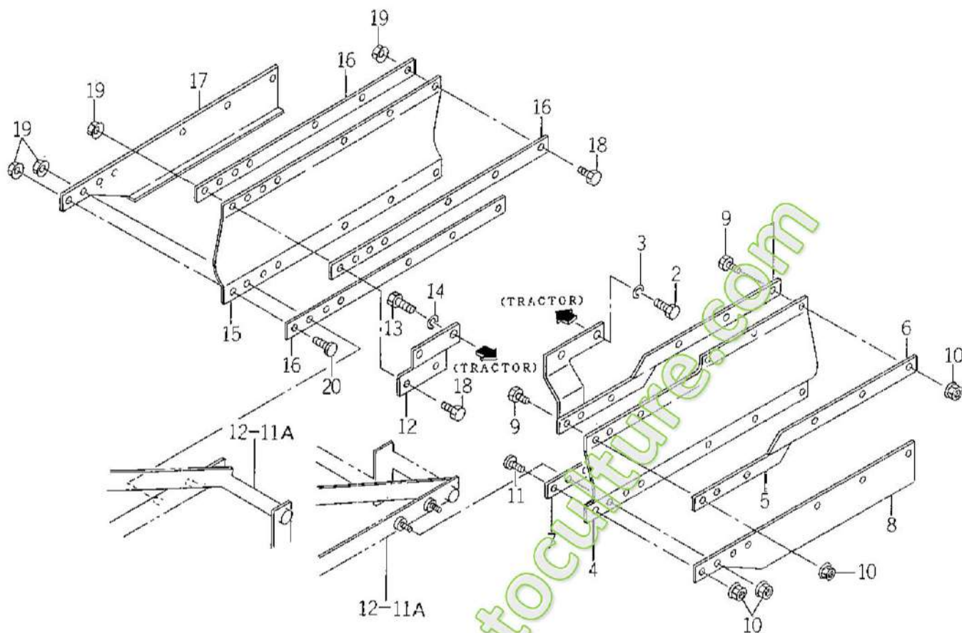
FIG. 15 PTO COVER SYSTEM (ME TYPE) (No.200001~)
