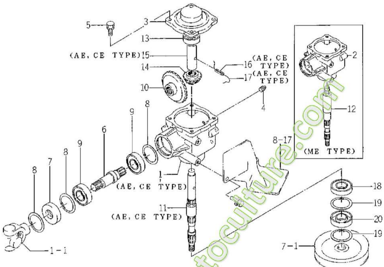
FIG. 6 CASE (BEVEL) SYSTEM (U TYPE)
