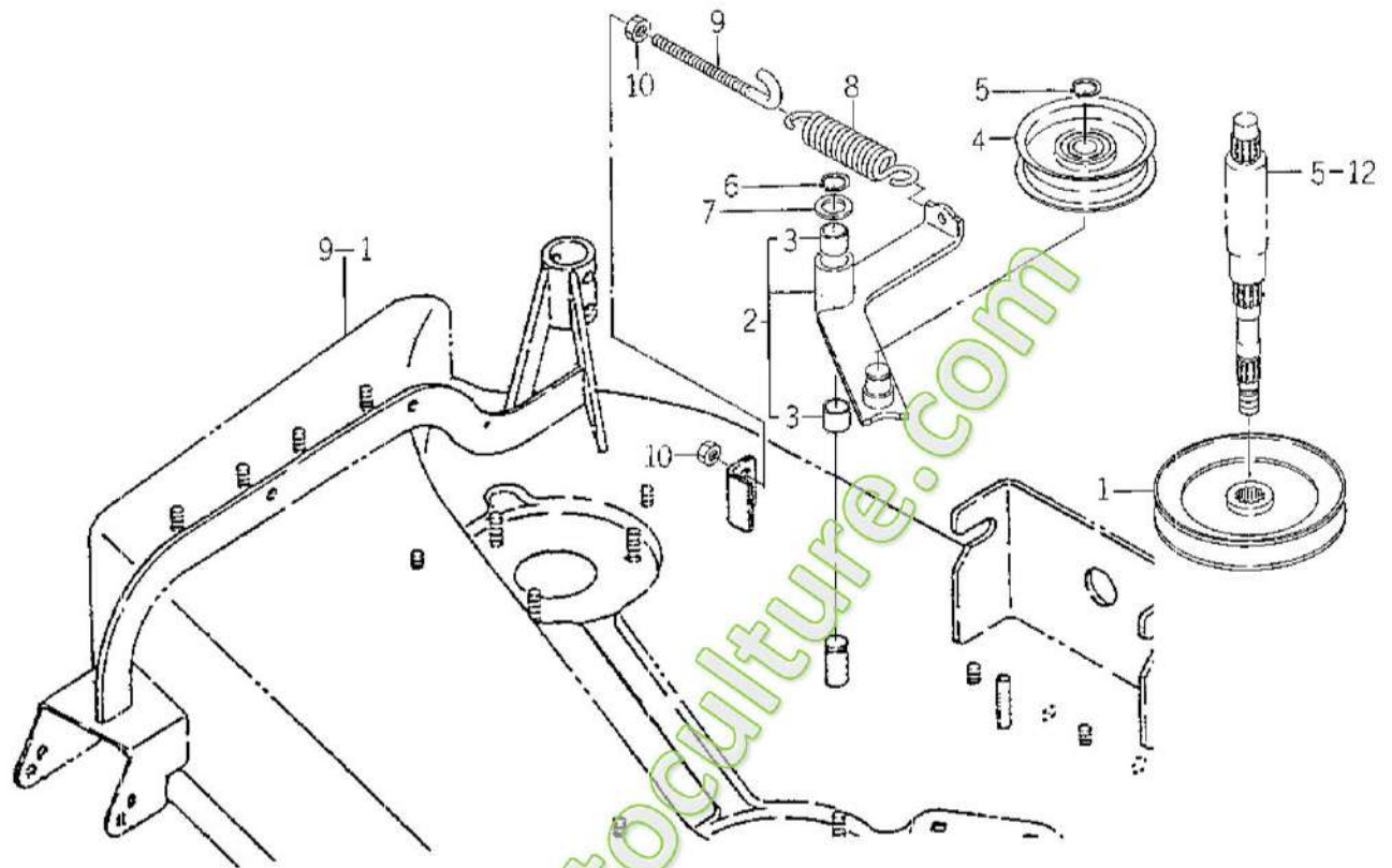
FIG. 7 PULLEY SYSTEM
