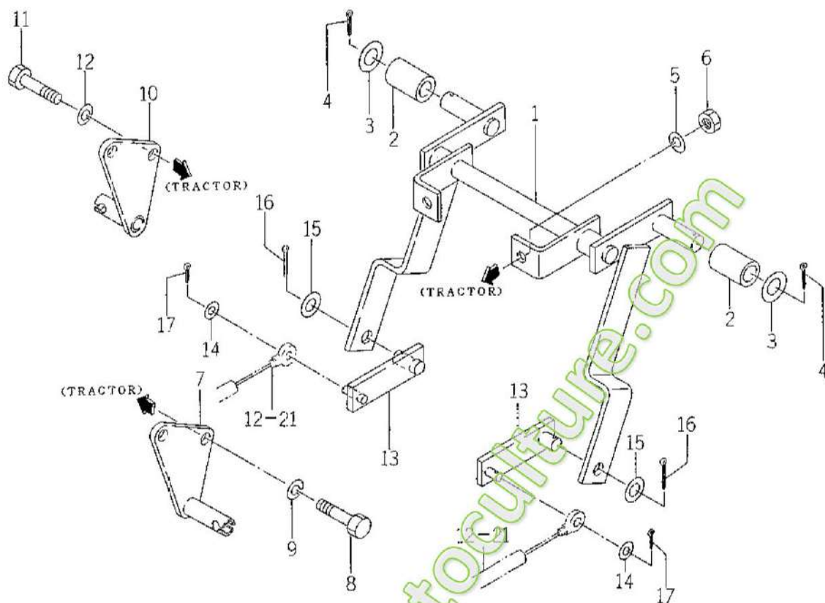
FIG. 13 LINK (REAR) SYSTEM (U15 TYPE)
