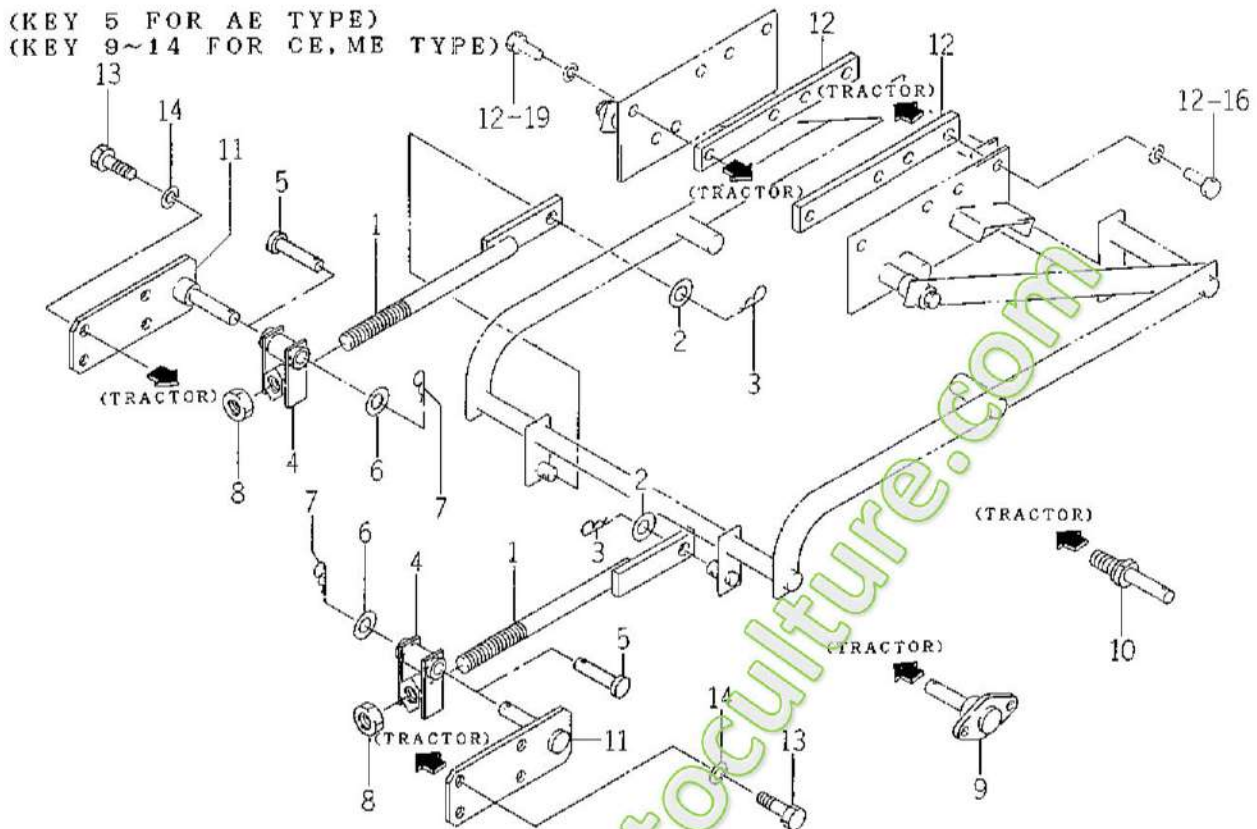
FIG. 11 LINK (FRONT) SYSTEM (U TYPE)
